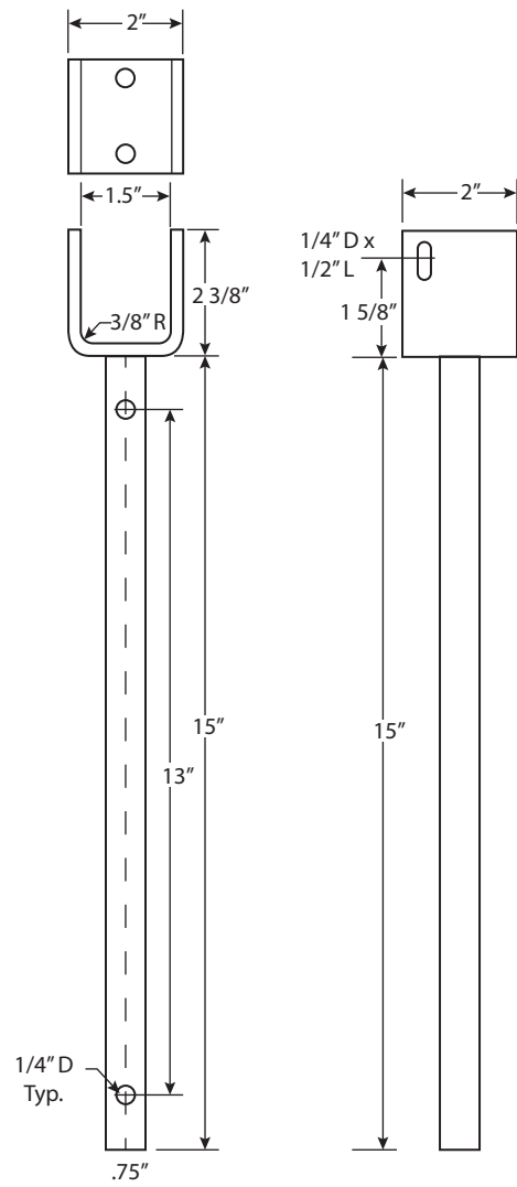
Invisible Shelf Bracket Round 15
